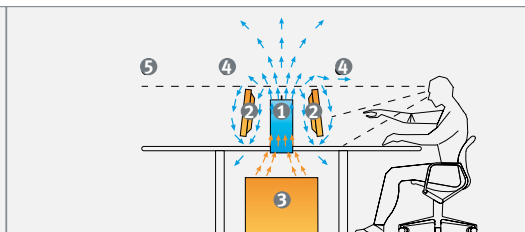
Air circulation with Cool-Top
